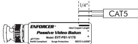
Figure 2: Measuring ideal copper length (1/4" or 6mm). Note: Use the convenient "Ideal Copper Length" gauge on the bottom of the balun.
