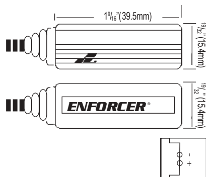
FIG. 6: Dimensions.
